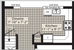
FIRST FLOOR KITCHEN OPTION B
