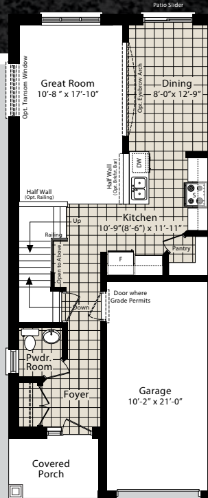
FIRST FLOOR JUNIPER (LEFT) 715 SQ. FT.
