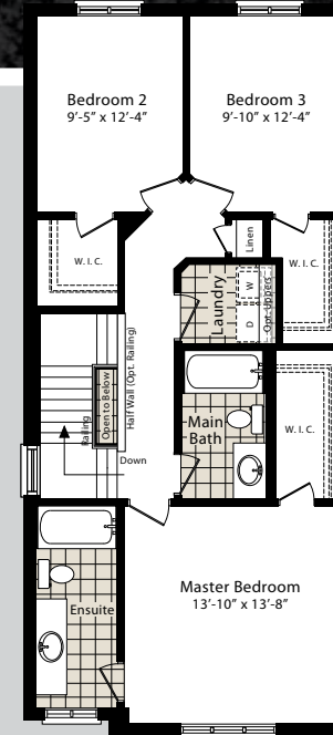
OPTION #1 MASTER ENSUITE JUNIPER (LEFT) 937 SQ. FT.
