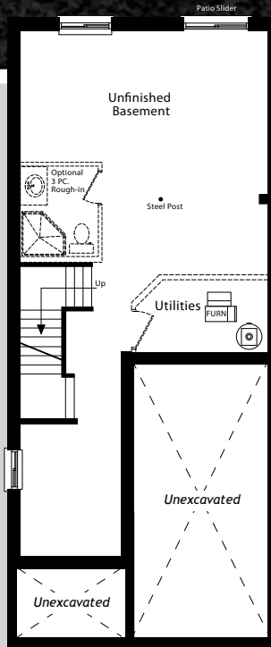
BASEMENT JUNIPER (LEFT)
