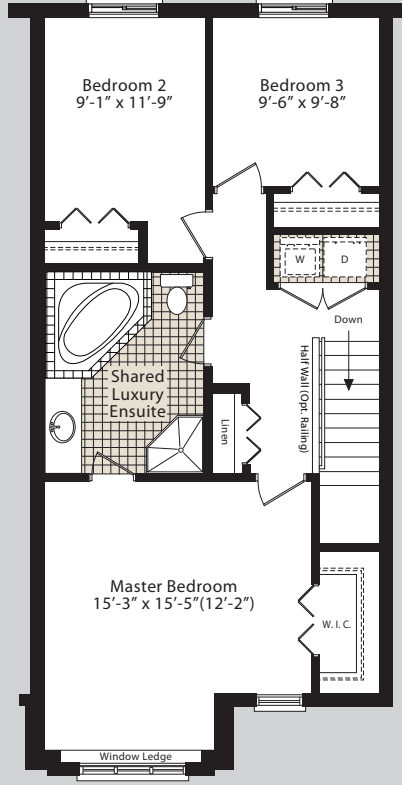
SECOND FLOOR SHARED LUXURY ENSUITE UNIT B51 & C59
