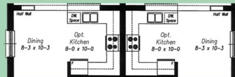
OPTIONAL KITCHEN LAYOUT
