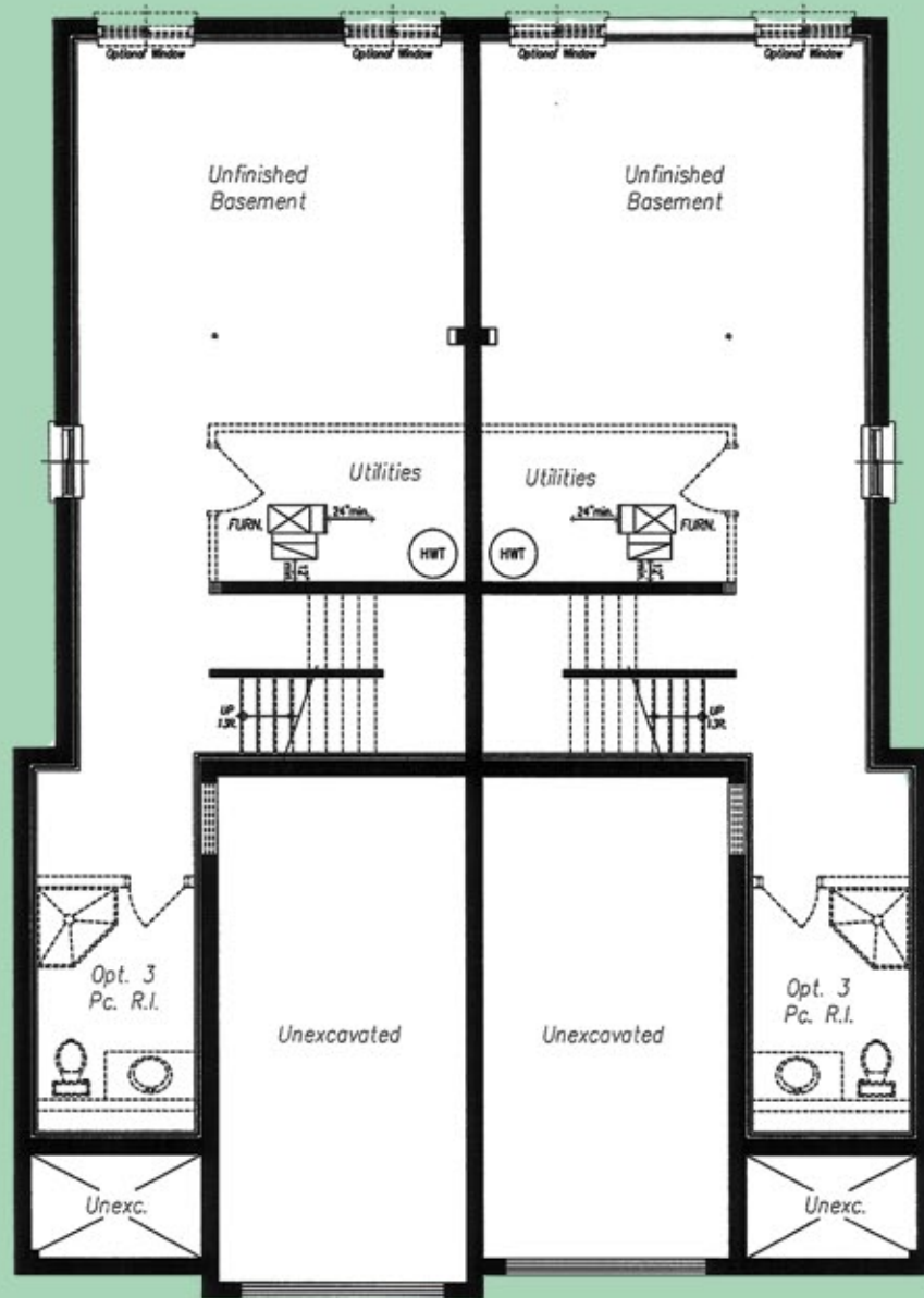
FOUNDATION PLAN
